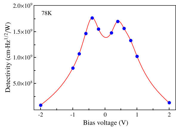
FIG. 4. The specific detectivity of the p -type QDIP for the response peak at 5 \mu\text{m} , plotted as a function of the bias.
