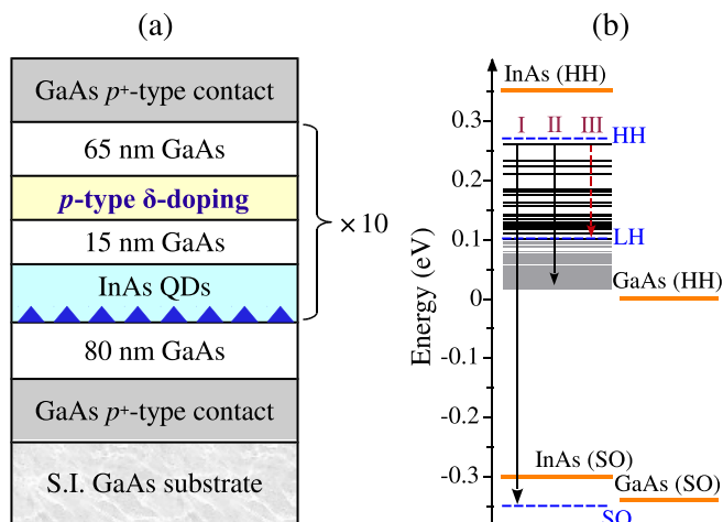
FIG. 1. (a) Schematic of the p -type QDIP structure. Free holes are introduced into QDs by \delta -doping above the QD layer. (b) Computed valence band structure of the QDs, where solid lines represent for hole states obtained by using an 8 \times 8 \mathbf{k} \cdot \mathbf{p} model. 18 The thick lines are the band edges. The dashed lines are the hole ground states of a QW, which has the same thickness as the QD height. The QW states were obtained using an effective-mass method, 20 with the potential confinement adopted from that of the QD in the growth direction through the dot center. 18,23 The states beyond the LH level become denser due to the larger hole effective mass and also to the LH confinement potential, which leads to a quasicontinuum of tenuously bound states. 22 Three transitions (I, II, and III) indicated contribute to the response as observed experimentally, where the transition III only observed at higher biases has the much weaker contribution compared to the other two.
